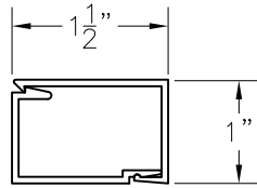
1 1/2" X 1" INTERIOR SNAP TRIM AND CLIP (PRODUCT CODE 6243)
