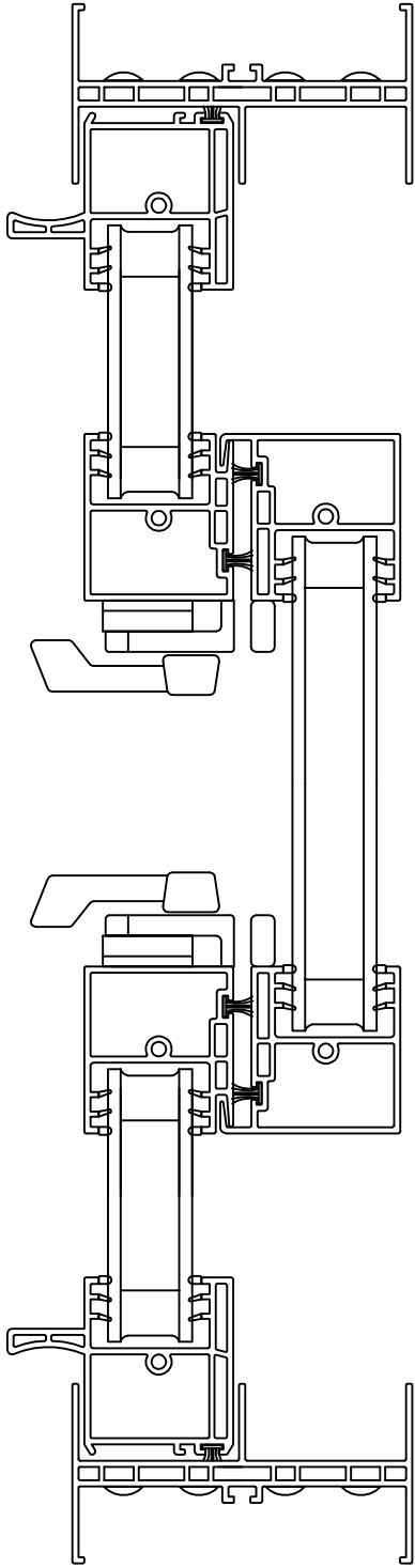
SECTION "C-C" NOT TO SCALE
