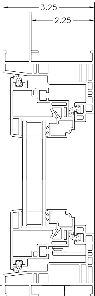
SECTION "A-A" NOT TO SCALE
