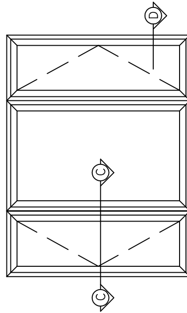
NUCON ® THREE-LITE CASEMENT NEW CONSTRUCTION WINDOW WELDED ASSEMBLY WITHOUT "J" CHANNEL
