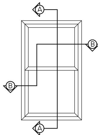
NUCON ® DOUBLE HUNG NEW CONSTRUCTION WINDOW WELDED ASSEMBLY WITH "J" CHANNEL
