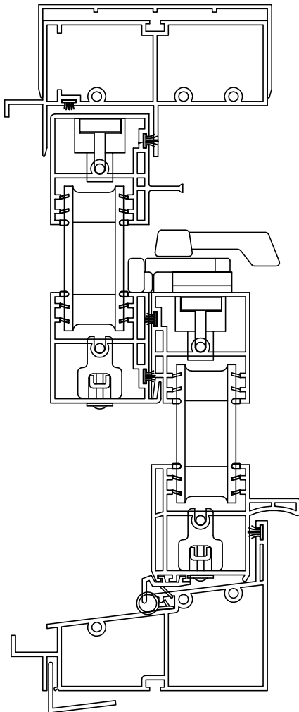
SECTION "A-A" NOT TO SCALE
